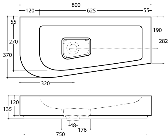
LAVABO Bacino dx e sx left or right installation
