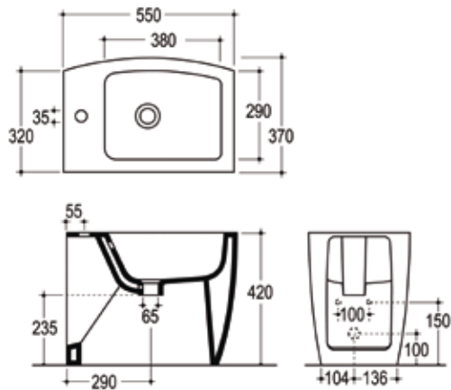
OLYBI Bidet monoforo Single-hole bidet
