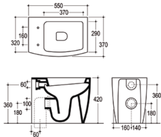
OLYVAP Vaso con scarico a parete Water closet with wall drain
